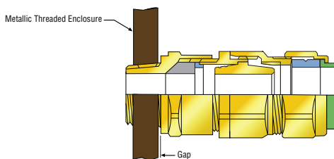
Tapered threaded gland into a threaded hole. Earth via entry thread when enclosure width is > greater than 4mm.
