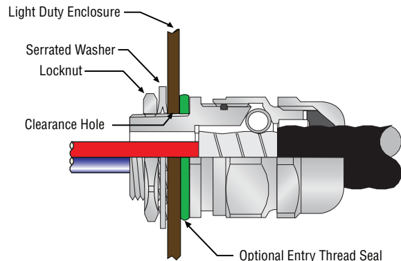
Taper threaded gland through clearance hole
