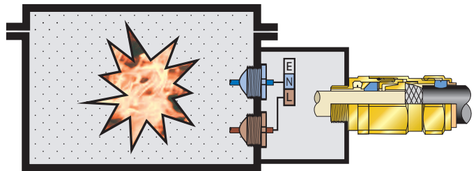
• Indirect Cable Entry - Ex d
