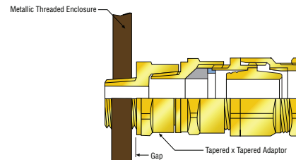
Taper x Taper adaptor through threaded hole. Earth via entry threads when enclosure is > 4mm.
